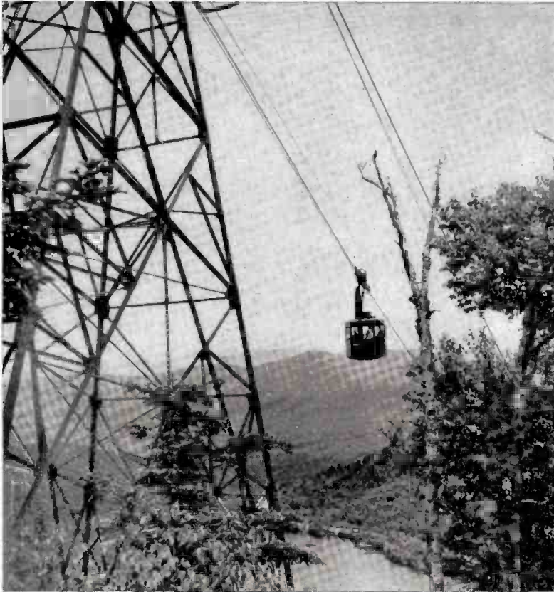
You'll Float Through The Air—For A Mile. This is a cable tramway for tourists that goes up Cannon Mountain at Franconia Notch in New Hampshire. The heavy wire ropes are well over a mile long, 1\frac{1}{4} inch in diameter and they weigh 28 tons apiece. The cable was made and installed by American Steel & Wire Division of United States Steel.
